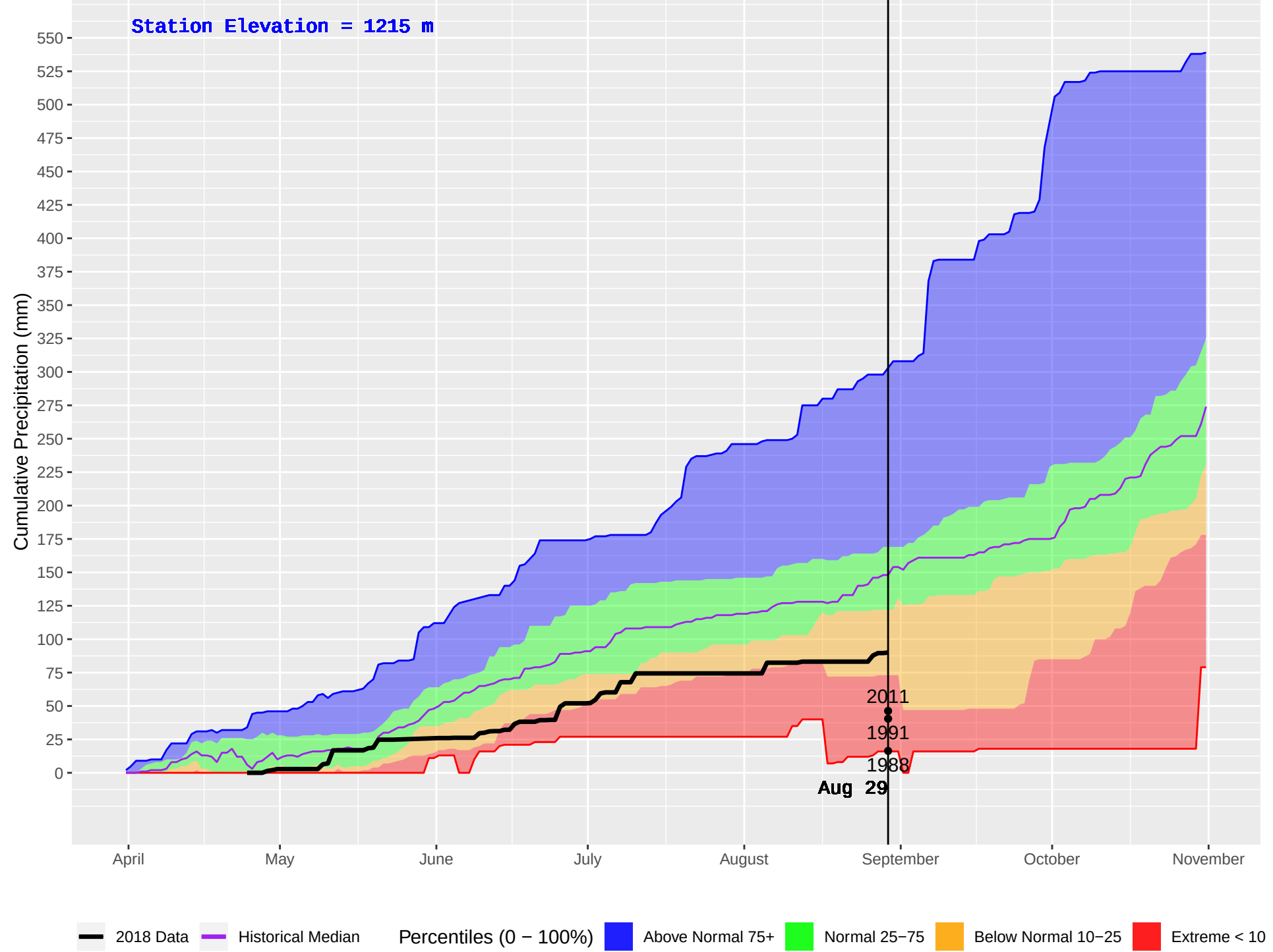
ALLISON PASS (317) : Historical (1987–2016) and Current (2018) Daily Cumulative Precipitation
