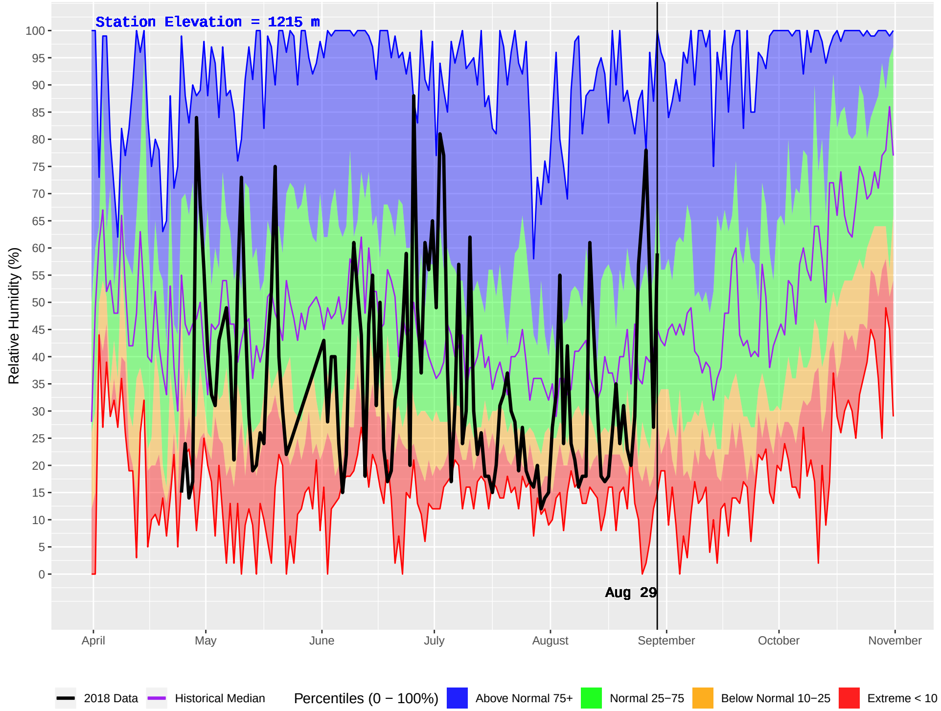
ALLISON PASS (317) : Historical (1987–2016) and Current (2018) Daily Relative Humidity
