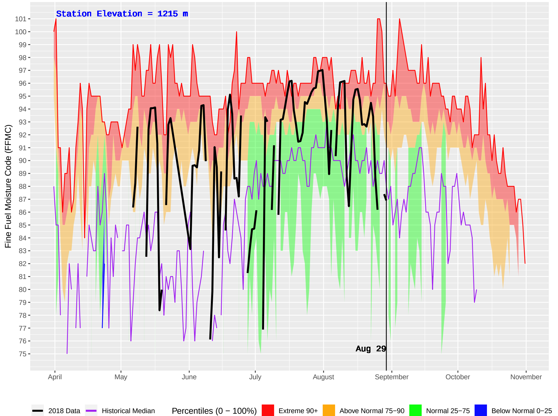
ALLISON PASS (317) : Historical (1987–2016) and Current (2018) Daily Fine Fuel Moisture Code (FFMC)
