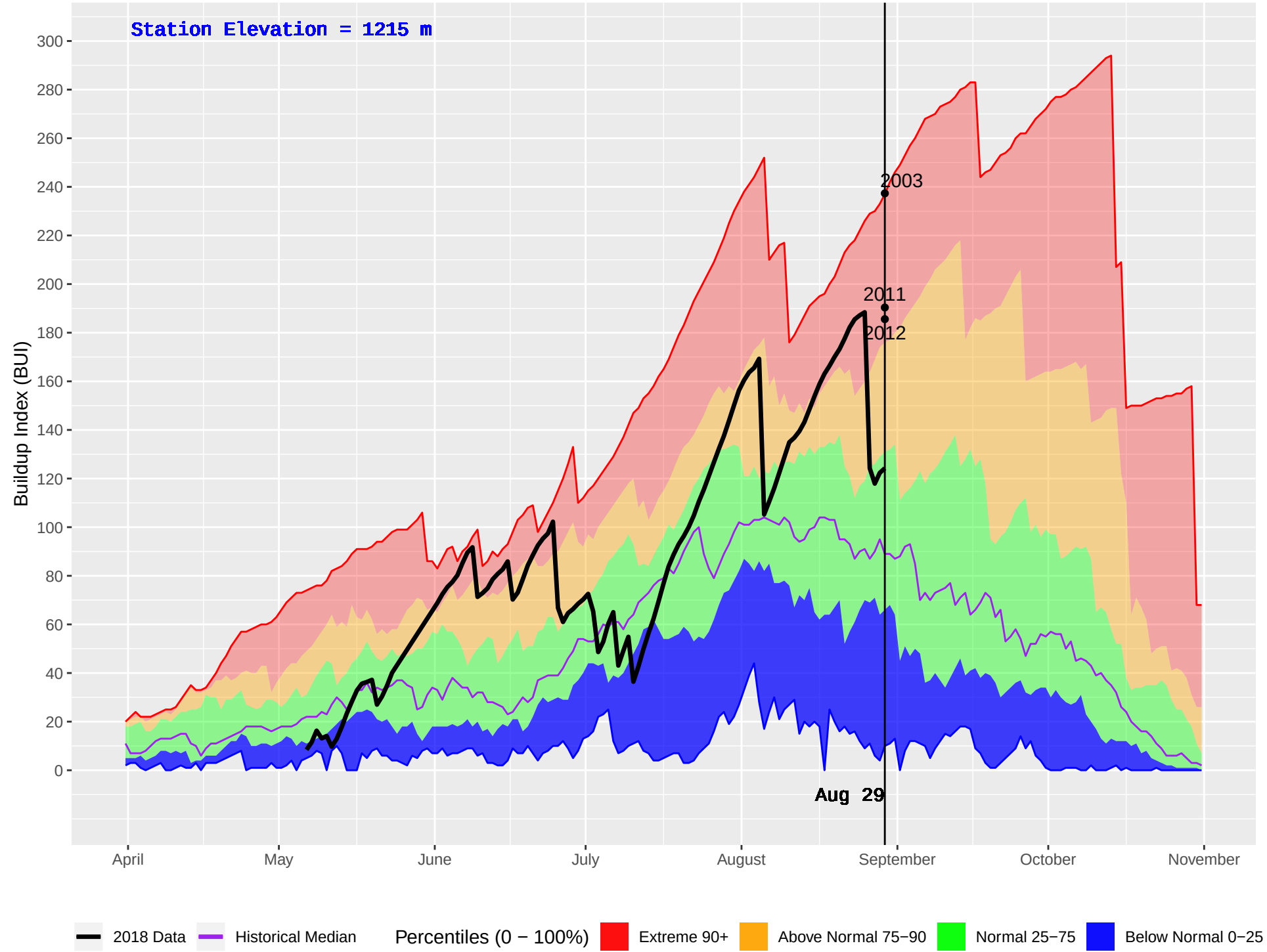
ALLISON PASS (317) : Historical (1987–2016) and Current (2018) Daily Buildup Index (BUI)
