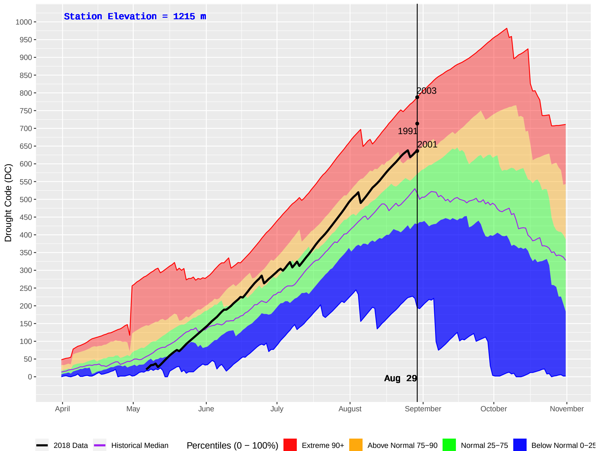
ALLISON PASS (317) : Historical (1987–2016) and Current (2018) Daily Drought Code (DC)
